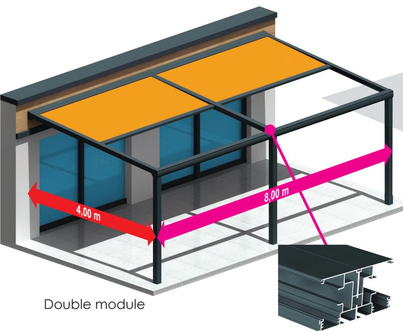
Fitting with double slide rail.
