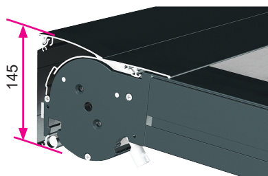
Operating space facade version
