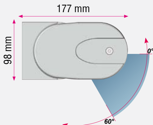
Installation façade / Wall installation
