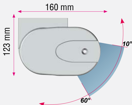
Installation plafond / Ceiling installation
